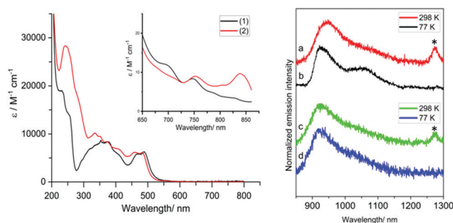
Fig. 3 Left: UV-vis absorption data for [Cr(bpi-1) 2 ]PF 6 (1) and [Cr(bpi-2) 2 ]PF 6 (2) including expansion of the long wavelength region. Emission data ( \lambda_{exc} = 430 \text{ nm} ; 850 nm cut-on longpass filter) for [Cr(bpi-1) 2 ]PF 6 (red, black) and [Cr(bpi-2) 2 ]PF 6 (green, blue) recorded in MeCN. ^1\Delta_g \rightarrow ^3\Sigma_g^- emission of oxygen highlighted by an asterisk.
