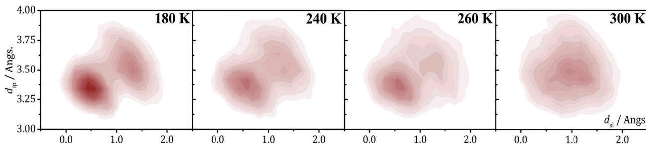
Fig. 19 2D-PDF's associated with the interplanar distance ( d_{ip} ) and the relative latitudinal slippage ( d_{sl} ) between adjacent NCBDTA radicals, as obtained from AIMD trajectories run at 180, 240, 260 and 300 K. Figure reprinted with permission of ref. 112.
