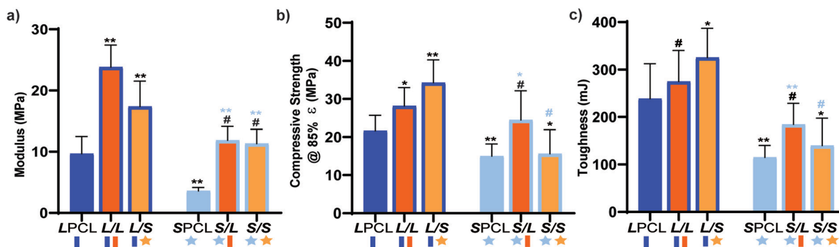
Fig. 4 Compressive mechanical properties were compared including (a) E , (b) CS , and (c) toughness; * p < 0.05 , ** p < 0.01 , # p > 0.05 . Note: the black color-coded statistics are compared to the LPCL and light blue color-coded statistics are compared to SPCL .
