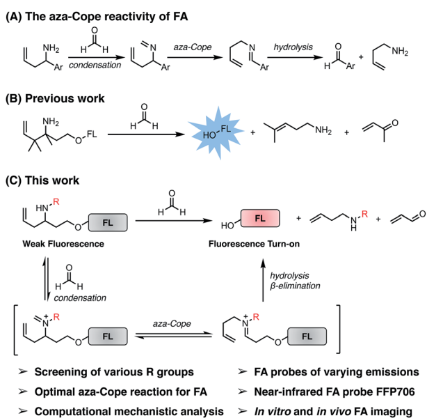
Fig. 1 The self-immolative aza-Cope strategy to construct fluorescent probes for detection and bioimaging of FA. (A) Previously reported aza-Cope reactivity of FA. (B) Previous work on the self-immolative aza-Cope strategy featuring the gem -dimethyl effect for enhanced aza-Cope reactivity to FA. (C) The present work focuses on systematic exploration of the effect of the N -substituent for identifying the optimal aza-Cope reaction with FA and provides a series of fluorescent probes for imaging FA in vitro and in vivo .
