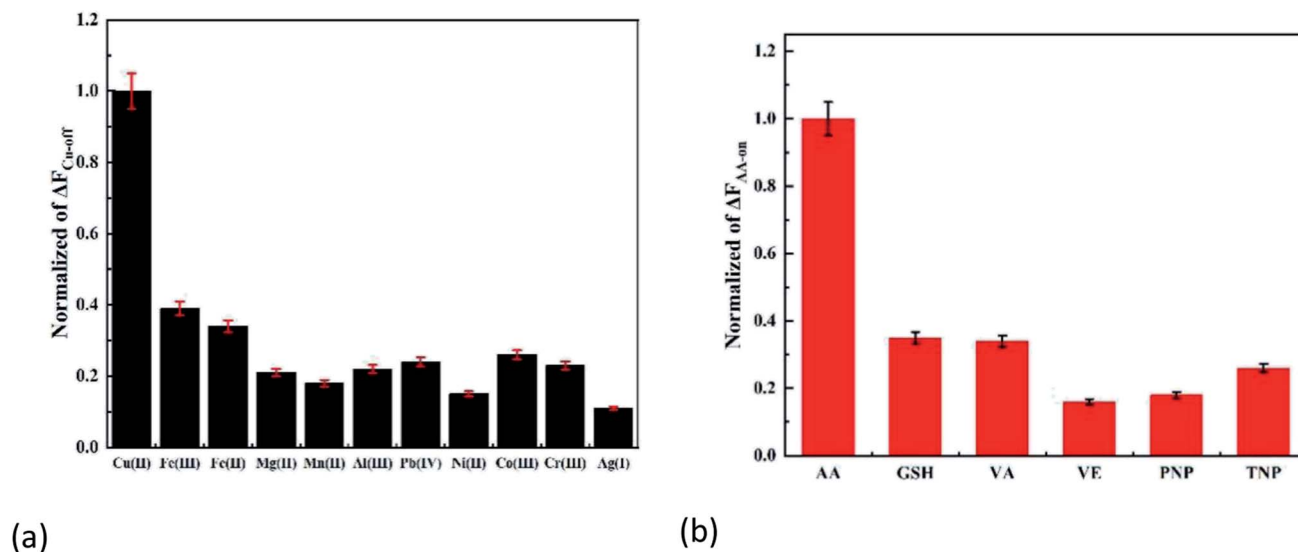
Fig. 5 Selectivity of (a) Cu(II) and (b) AA.
