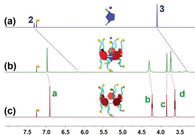
Fig. 1 Partial ^1\text{H} NMR spectra (600 MHz, \text{CDCl}_3 , room temperature): (a) G1 ; (b) BrP5 (10.0 mM) and G1 (10.0 mM); and (c) BrP5 . The peaks marked with orange dots are ascribed to \text{CDCl}_3 -d.
