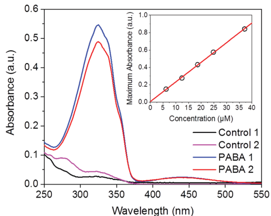
Fig. 5 Quantification of the PABA solvent-extracted from test and control membranes. UV/Vis absorption spectra of ethanol washings after two days for two control samples (black and pink lines) and two test samples (blue and red lines) are shown. The inset shows the Beer–Lambert calibration plot for PABA in ethanol ( \lambda = 324 nm).
