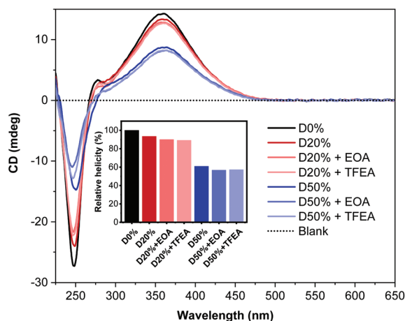
Fig. 7 CD (THF, 0.5 mg mL -1 ) spectra of D0%, D20%, and, D50% before and after treatment with EAO or TFEA and purification by dialysis. The inset shows the helicity (CD at \lambda = 360 nm) of the copolymers compared to D0%.
