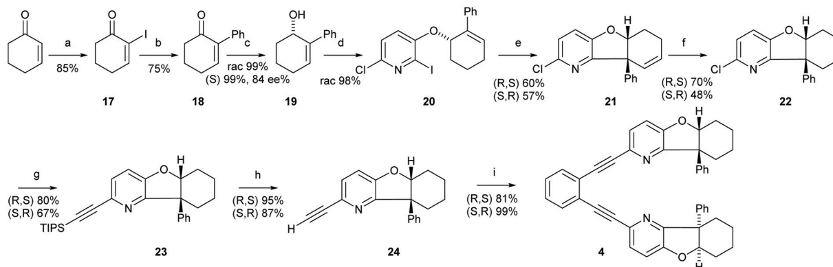
Scheme 3 The synthetic route to ligand 4 . Reagents and conditions: (a) \text{I}_2 , DMAP, \text{K}_2\text{CO}_3 , \text{H}_2\text{O}/\text{THF} (1:1), r.t., 2 h.; (b) \text{Pd/C} , \text{PhB}(\text{OH})_2 , \text{Na}_2\text{CO}_3 , \text{DME}/\text{H}_2\text{O} (1:1), r.t., 18 h; (c) \text{CeCl}_3 , \text{NaBH}_4 , MeOH, 0 °C to r.t. in 2 h; (d) 6-chloro-2-iodopyridine-3-ol, DIAD, \text{PPh}_3 , toluene, r.t., 3 days; (e) \text{Pd}(\text{PPh}_3)_2\text{Cl}_2 , \text{Ag}_2\text{CO}_3 , \text{NEt}_3 , toluene, 110 °C, 24 h; (f) \text{Rh/C} , \text{H}_2 , MeOH; (g) trans - [\text{PdCl}_2(\text{CH}_3\text{CN})_2] , XPhos, \text{Cs}_2\text{CO}_3 , \text{CH}_3\text{CN} , 85 °C, 8 h; (h) (1) NuB4F, THF, 0 °C, 2 h, then (2) 1,2-diiodobenzene, \text{Pd}_2(\text{dba})_3 , \text{PPh}_3 , \text{CuI} , \text{NEt}_3 , 45 °C, 20 h. For details, see the ESI.†
