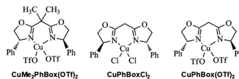
Scheme 17 Copper(II) complexes with bis(oxazoline) ligands; OTf = trifluoromethylsulfonate.
