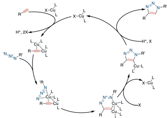
Scheme 33 Reaction mechanism of the CuAAC, X: mostly \text{SO}_4^{2-} , \text{I}^- , \text{Br}^- , \text{Cl}^- , \text{PF}_6^- , L = ligand such as THTPA, TBTA.
