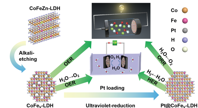
Scheme 1 Schematic illustration of the synthesis process for multifunctional Pt@CoFe v -LDH.
