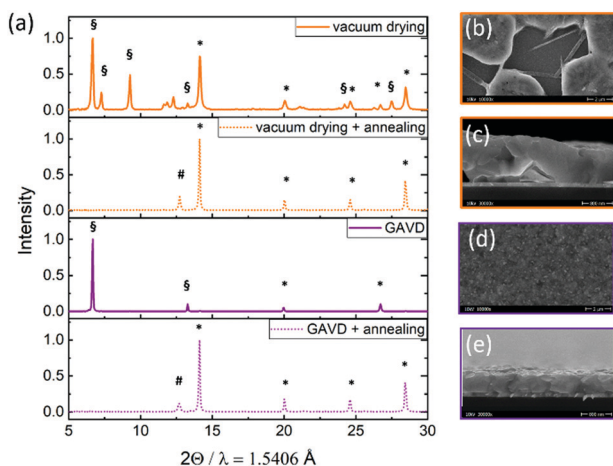
Fig. 3 (a) X-ray diffraction patterns of MHP films measured directly after vacuum and GAVD treatment, and collected after temperature annealing at 100 °C. * mark the reflexes of the perovskite tetragonal phases. # marks the \text{PbI}_2 reflex. § marks the \text{MA}_2\text{DMSO}_2\text{Pb}_3\text{I}_8 intermediate phase according to Cao et al. 33 Scanning electron microscope (SEM) images of vacuum-dried (c and b) and GAVD-treated (d and e) samples after temperature annealing.
