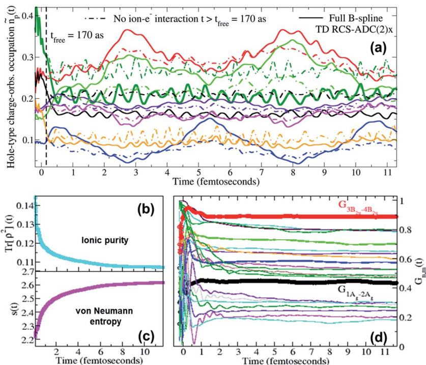
Fig. 5 (a) Time-dependent hole-occupation numbers \tilde{n}_p(t) (eqn (11)) of the "occupied" natural charge orbitals triggered by attosecond ionisation of the C 4 H 4 N 2 molecule in the pump step; full lines: full TD RCS-ADC(2)x results; dashed lines: results obtained by switching off the residual interaction between the parent-ion and the photoelectron at t_{\text{free}} = 170 as after ionisation. Time evolution of (b) the purity \text{Tr}[\rho^2](t) and (c) the von Neumann entropy of entanglement s(t) of the bipartite ion–photoelectron system after pump ionisation of the C 4 H 4 N 2 molecule. (d) Time evolution, upon ionisation by the pump laser pulse, of the degrees of coherence G_{m,n}(t) of the pairs of ionic states mostly contributing to the density-matrix purification (see Fig. 6); the time evolution of the G_{1A_g, 2A_g}(t) (black curve) and G_{3B_{2u}, 4B_{2u}}(t) (red curve) coherences, mostly contributing to the pump-triggered charge dynamics, are highlighted.
