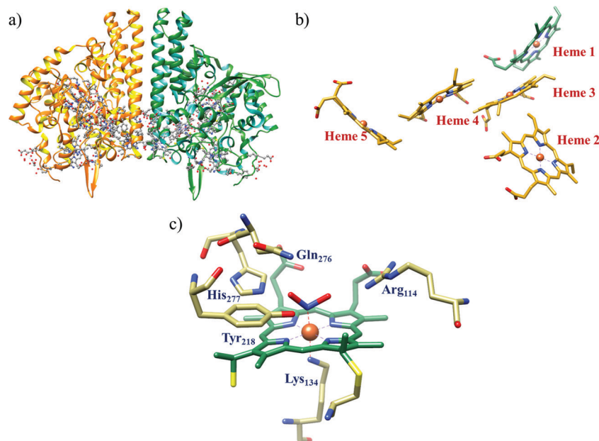
Fig. 10 (a) Three-dimensional structure of the Wolinella succinogenes CcNiR homodimer, the momomers are shown in different colours (with yellow and green ribbon colour), (b) arrangement of hemes (1–5) in the monomer with green ribbons; the five heme c are numbered according to their attachment to the protein chain. Heme 1 contitutes the enzyme active site. (c) Nitrite bound active site structure. (a) and (b) are based on PDB file 1FS7 182 and (c) is based on PDB file 2E80. 175
