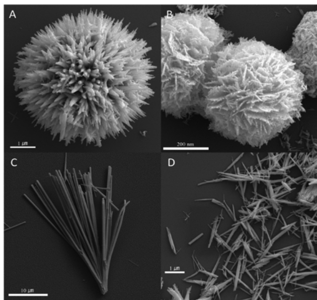
Fig. 2 SEM micrographs of, \text{Bi}_{13}\text{S}_{18}\text{I}_2 -a (A) and \text{Bi}_{13}\text{S}_{18}\text{I}_2 -b (B) BiSI-a (C), BiSI-b (D).
