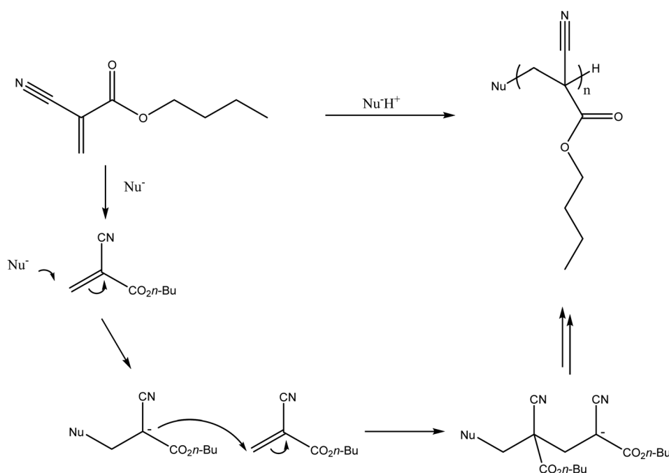
Fig. 1 In situ polymerisation of N -butyl-2-cyanoacrylate ( n BCA). (Nu - refers to a nucleophilic species, which would most commonly be water in the case of delivery into the blood stream).
