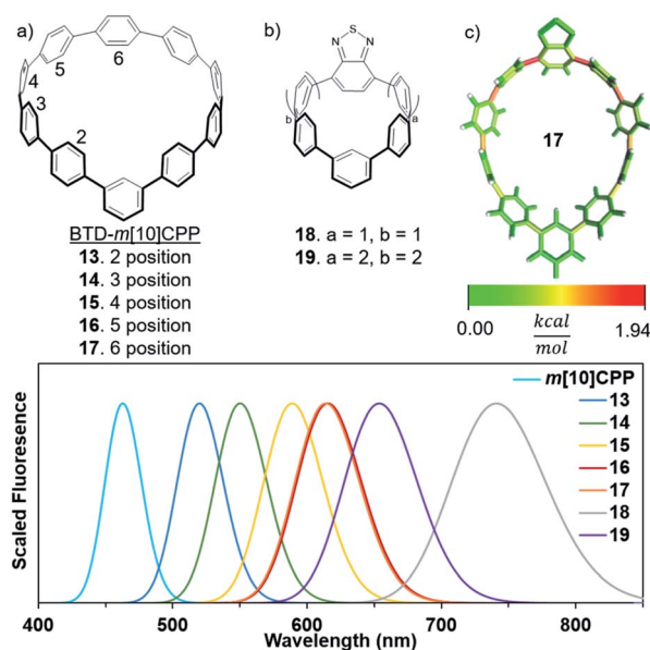
Fig. 5 Calculated emission of (a) BT unit in different positions of m [10]CPP, and (b) smaller CPPs to analyze strain effects on acceptor properties. (c) Strain analysis of BTD incorporated m [10]CPP.
