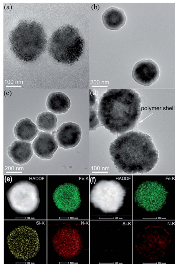
Fig. 1 TEM images of (a) \text{Fe}_3\text{O}_4 NPs, (b) \text{Fe}_3\text{O}_4@/\text{SiO}_2 , (c) \text{Fe}_3\text{O}_4@/\text{SiO}_2@/\text{Poly}(\text{L-Trp}) , and (d) yolk-shell \text{Fe}_3\text{O}_4@/\text{Poly}(\text{L-Trp}) . (e) and (f) show the TEM elemental mapping images of \text{Fe}_3\text{O}_4@/\text{SiO}_2@/\text{Poly}(\text{L-Trp}) and yolk-shell \text{Fe}_3\text{O}_4@/\text{Poly}(\text{L-Trp}) , respectively.
