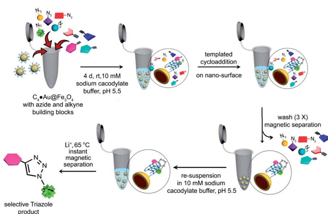
Fig. 4 Schematic representation of the target guided synthetic approach using i-motif magnetic nanotemplates ( c-MYC C_4 \cdot Au@Fe_3O_4 & BCL2 C_4 \cdot Au@Fe_3O_4 ) for in situ formation of potent binders.
