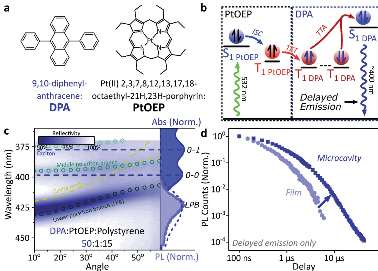
Fig. 2 Sensitized photon up-conversion. (a) Molecular structures of active components used in photon up-conversion system. (b) Simplified schematic of photon up-conversion, details in main text. ISC: intersystem crossing, TET: triplet energy transfer, TTA: triplet-triplet annihilation. (c) Reflectivity map of photon up-conversion blend within a Ag-Ag microcavity. Comparison with absorption spectrum (upper right, dark blue) and transfer matrix modelling (lines, circles) confirms strong coupling, characterised by anti-crossings at the 0-0 and 0-1 energies (dashed). Details of transfer matrix model in ESI,† Methods. All emission comes from the lower polariton branch (LPB), whether excitation is resonant with diphenylanthracene (355 nm, lower right, dashed spectrum) or PtOEP (532 nm, lower right, shaded spectrum). Emission is collected with a NA = 0.76 lens and thus effectively integrates along the entire dispersion ( \pm 45^\circ ). (d) Decay kinetics of diphenylanthracene/exciton-polariton emission following excitation of PtOEP at 532 nm reveal enhanced lifetime in microcavity (dark) vs. bare film (light). All emission on these timescales arises from triplet-triplet annihilation. Incident power (film: 50 \mu W, microcavity: 150 \mu W) yields \sim 2\times greater excitation density in the microcavity, which should result in faster intrinsic depletion of triplets.
