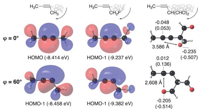
Fig. 5 The frontier in-plane \pi -orbital in 1-fluoro-2-butyne ( \text{R} = \text{CH}_2\text{F} ) is stabilized more than in 2-butyne ( \text{R} = \text{CH}_3 ) due to a hyperconjugative \sigma_{\text{C-F}}^* - \pi overlap. For \text{R} = \text{CH}(\text{CHO})_2 , electrostatic interactions are presumed to be responsible for the low bending force. Additionally, Hirshfeld (NPA) charges are shown.
