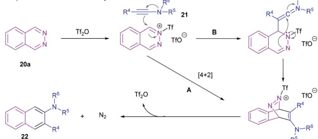
Scheme 5 Tf 2 O-catalyzed [4 + 2] benzannulation to synthesize 2-aminonaphthalenes and 2-aminoanthracenes.
