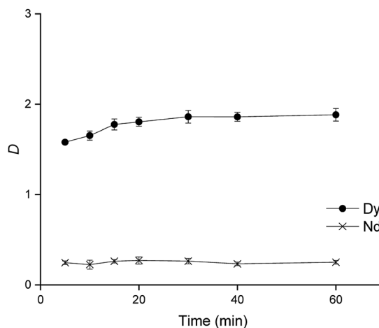
Fig. 3 Influence of time on the separation of Nd(III) and Dy(III) from a 2.5 M \text{CaCl}_2 matrix to an organic phase composed of 40 wt% Cyanex 923, 60 wt% [C101][SCN] shaking speed: 2000 rpm at 25 °C.
