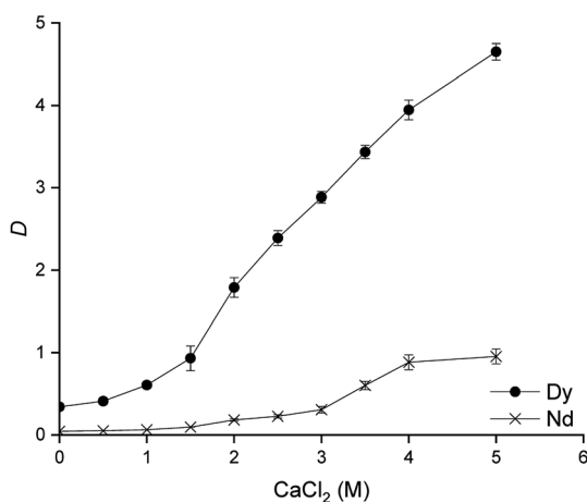
Fig. 2 Effect of the \text{CaCl}_2 concentration on the separation of Nd(III) and Dy(III). Equilibration time: 60 min. Shaking speed: 2000 rpm at 25 °C, 40 wt% Cyanex 923 in [C101][SCN].
