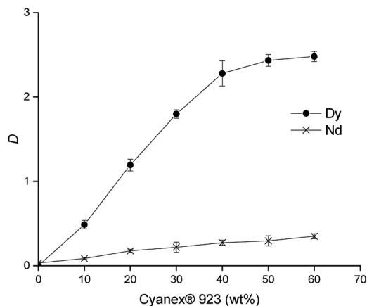
Fig. 1 Effect of the concentration of Cyanex® 923 diluted in [C101][SCN] on the separation of Nd(III) and Dy(III) in 2.5 M \text{CaCl}_2 . Equilibration time: 60 min. Shaking speed: 2000 rpm at 25 °C.
