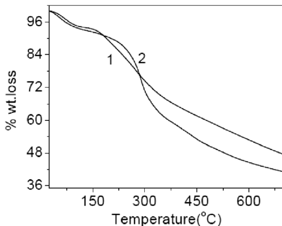
Fig. 19 Thermogravimetric curves of polyanthranilic acid obtained by: 1 – the classical method and 2 – interface polymerization. Reproduced with permission from ref. 80.
