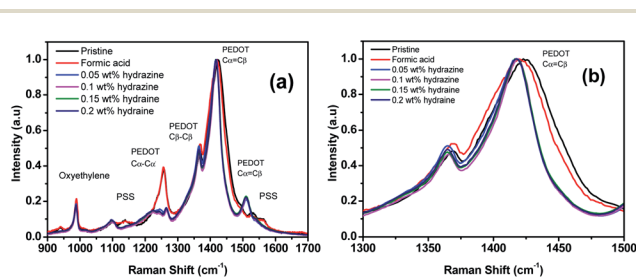
Fig. 7 (a) Raman spectra of the PEDOT:PSS films before and after treatment with formic acid and formic acid-hydrazine. (b) The zoom-in spectra for the wavenumbers ranging from 1300 to 1500 \text{cm}^{-1} .
