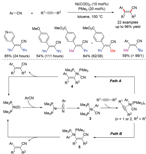
Scheme 3 Ni-Catalyzed arylation of alkynes.
