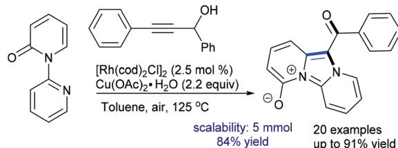
Scheme 104 Alkenylation and concomitant intramolecular annulation.
