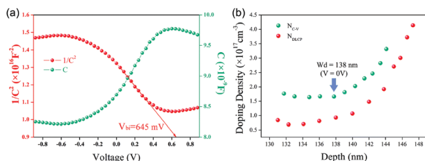
Fig. 12 (a) The C - V (green) and 1/C^2 - V (red) curves for the GeSe solar cell tested at room temperature under dark conditions. (b) C - V profiling and DLCP profiling for the GeSe solar cell. Reprinted with permission from ref. 56. Copyright 2019, Royal Society of Chemistry.
