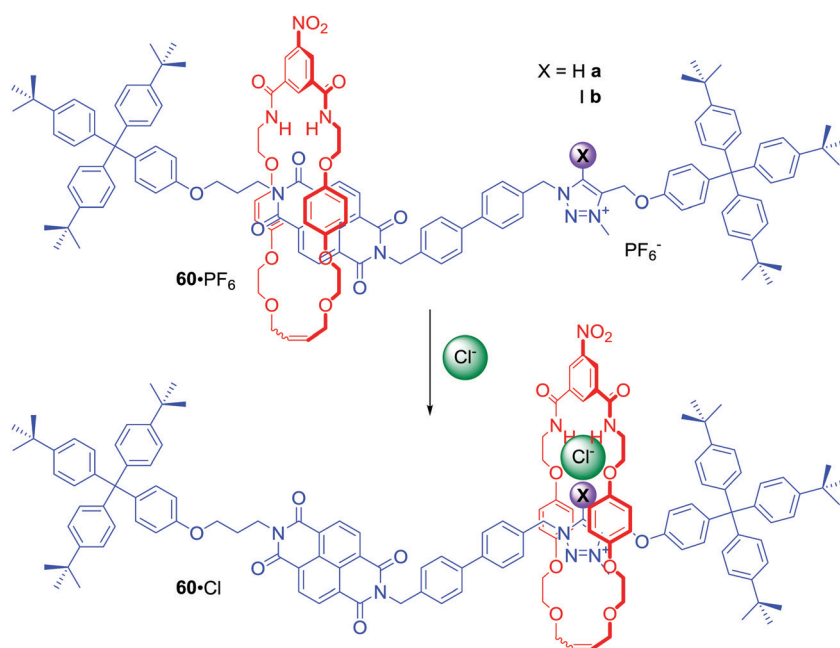
Scheme 3 Chloride-driven shuttling of [2]rotaxane.
