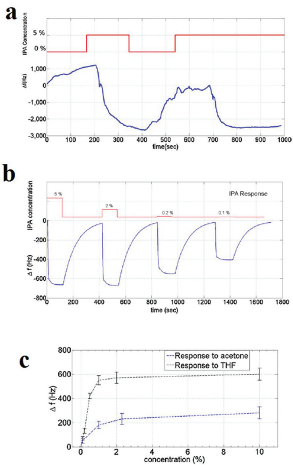
Fig. 13 Application of HKUST-1 thin film in the detection of volatile molecules by gravimetric sensing. (a) The response of the drop-casted film to 5% IPA. (b) Response of the electrospayed film to IPA. Responses of the sensor with electrospayed film to different concentrations of (c) acetone and THF. Reproduced with permission from ref. 313.
