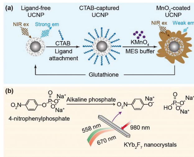
Fig. 4 Yb-Based UCNPs for biosensing. (a) Schematic design of surface modification and GSH detection by using the \alpha -NaYbF 4 :Tm (1 mol%)-@CaF 2 core-satellite UCNPs. (b) Schematic design for screening the activity of alkaline phosphatase by using the KYb 2 F 7 UCNPs. Reprinted with permission from ref. 30 and 33. Copyright 2018 the Royal Society of Chemistry and 2014 Springer Nature, respectively.
