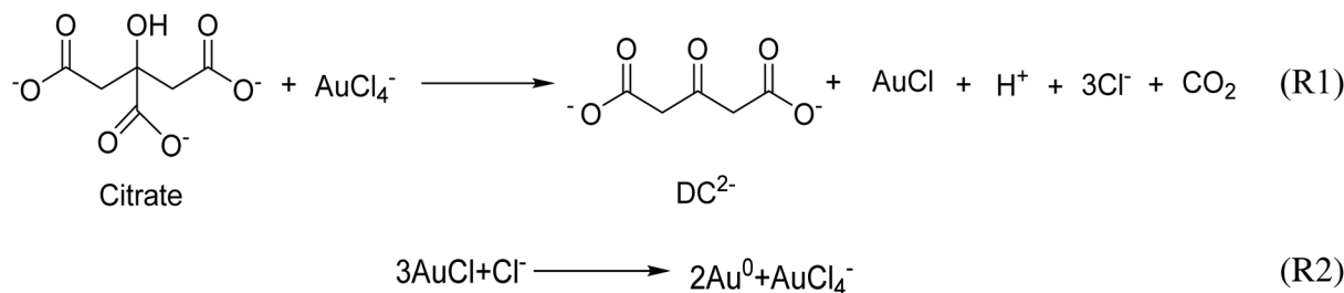
Scheme 1 The accepted mechanism for Turkevich protocol, consisting of the initial redox reaction (R1) and the disproportionation reaction (R2).
