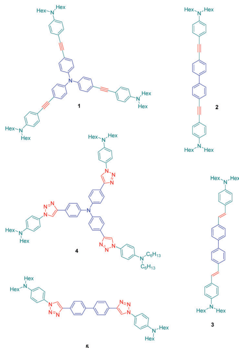
Fig. 1 Structures of triazole-based dyes 4 and 5 and their alkyne/alkene bridged analogues 1–3.
