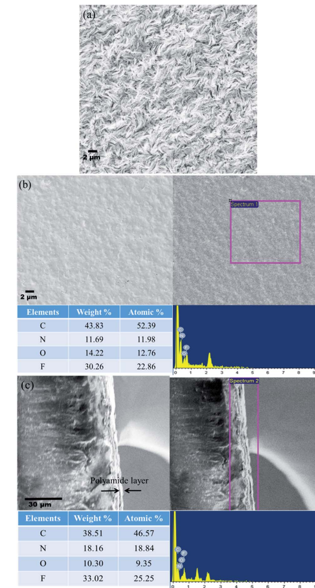
Fig. 9 (a) SEM micrograph of the control membrane indicating a spherulitic morphology, (b) surface morphology of the PA-GQD membrane with EDX analysis, and (c) cross-sectional morphology of the PA-GQD membrane with EDX analysis.
