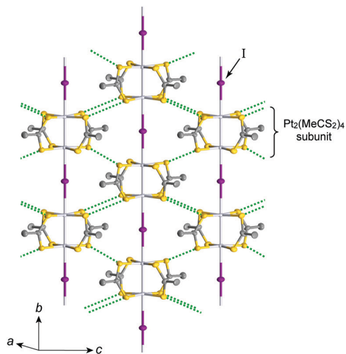
Fig. 4 Crystal structure of \text{Pt}_2(\text{MeCS}_2)_4\text{I} at room temperature, 18,19 where green dotted lines show heteroatomic \text{S} \cdots \text{S} contacts between adjacent chains. Hydrogen atoms are omitted for clarity.
