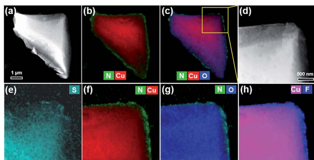
Fig. 4 High-angle annular dark field scanning TEM (HAADF-STEM) imaging (a, d) and corresponding EDX elemental maps (b and c, e–h).
