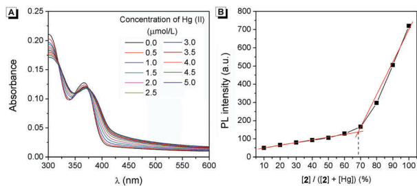
Fig. 7 (A) Absorption spectra of 10 \mu\text{mol L}^{-1} 2 upon the addition of \text{Hg(II)} . (B) Job's plot data for evaluating the stoichiometry of the 2 - Hg-2 complex. The total concentration of 2 and \text{Hg(II)} was kept at 20 \mu\text{mol L}^{-1} . 99% water/DMSO ( v/v ) at pH 7.0 controlled by 10 \text{mmol L}^{-1} Tris solution was used. Excitation and emission were performed at 368 nm and 445 nm, respectively.
