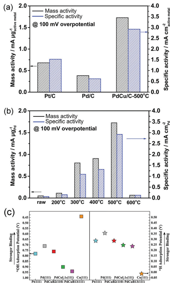
Fig. 12 (a) and (b) Comparison of HOR mass and specific activity (MA and SA) of Pt/C, Pd/C, and PdCu/C at overpotential of 100 mV in H 2 -saturated 0.1 M KOH electrolyte. (c) Equilibrium adsorption potentials (vs. RHE) for *H (1/6 ML) and *OH (1/3 ML) on Pt, Pd, bcc-PdCu (B2 phase), and fcc-PdCu (L1 0 and B13 phases) terrace surfaces. The three PdCu surfaces shown here are covered by 1 mL Pd. Adapted with permission from ref. 148. Copyright 2018, Royal Society of Chemistry.
