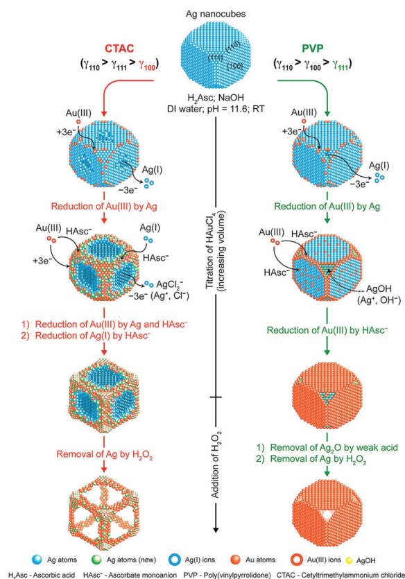
Fig. 7 Schematic illustration describing the mechanisms proposed for the deposition of Au and Ag atoms on Ag NCs when HAuCl_4 is titrated into an aqueous suspension of Ag NCs in the presence of H_2Asc , NaOH, and CTAC (left) or PVP (right) at an initial pH of 11.6. Adapted with permission from ref. 101. Copyright 2017, American Chemical Society.
