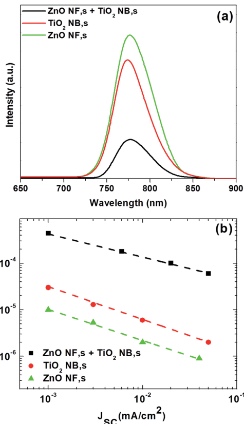
Fig. 4 (a) Steady-state PL spectra of perovskite absorber layers formed on different ETMs, and (b) electron lifetime for the PSCs based on different ETMs, respectively.
