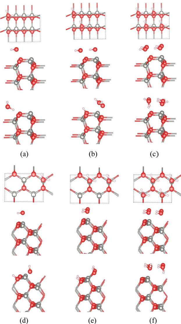
Fig. 10 Top and side views for the initial geometries, and side views of the final geometries, for WZ(10 \bar{1}0 ) films of ZnO with (a) 25%, (b) 50% and (c) 100% water coverage. Top and side views of ZB(110) for ZnO with (d) 25%, (e) 50% and (f) 100% water coverage. In (b), half of the water molecules dissociate. In (d and e), the water dissociates forming H + and OH - . In (a, c and f), there is molecular adsorption.
