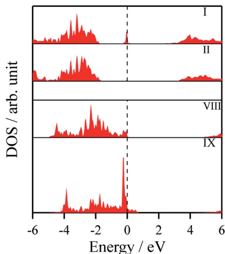
Fig. 7 Partial density of states (PDOS) per layer for polar ZB(111) for ZnS with 9 layers. A similar figure but expanded with PDOS plots for all the layers are given in the ESI.†
