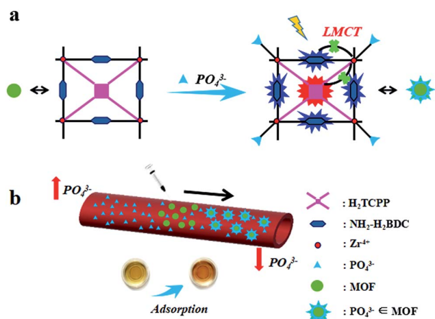
Scheme 1 Schematic diagram for the treatment of hyperphosphatemia based on Zr(IV) -MOFs. (a) Proposed mechanism of the fluorescence nanosensor for phosphate; (b) reduced levels of phosphate by MOFs for highly efficient treatment of hyperphosphatemia.
