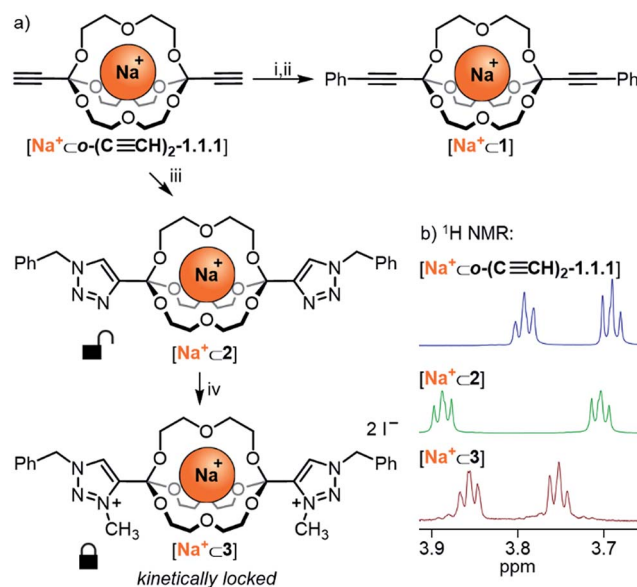
Scheme 3 Post-functionalization of orthoester cryptands. (a) Reaction conditions: (i) [ Na + ⊂ o-(C≡CH) 2 -1.1.1 ] (11.8 μmol, 1.0 equiv.), iodobenzene (23.6 μmol, 2.0 equiv.), NEt 3 (35.4 μmol, 3.0 equiv.), CuI (0.12 μmol, 0.01 equiv.), Pd(PPh 3 ) 4 (0.12 μmol, 0.01 equiv.), THF, 40 °C, 4 d, 94%. (ii) 1 (9.28 μmol, 1.0 equiv.), NaBARf (9.28 μmol, 1.0 equiv.), CH 3 CN, r.t., 5 min, quant. (iii) [ Na + ⊂ o-(C≡CH) 2 -1.1.1 ] (11.0 μmol, 1.0 equiv.), benzyl azide (22.0 μmol, 2.0 equiv.), Cu(MeCN) 4 PF 6 (0.11 μmol, 0.01 equiv.), TBTA (0.11 μmol, 0.01 equiv.), MeOH, 70 °C, 24 h, 92%. (iv) [ Na + ⊂ 2 ] (3.9 μmol, 1.0 equiv.), MeI (excess), MeCN, 70 °C, 3 d, 83%. (b) Partial 1 H NMR stacked plot (500 MHz, 298 K, CD 3 CN).
