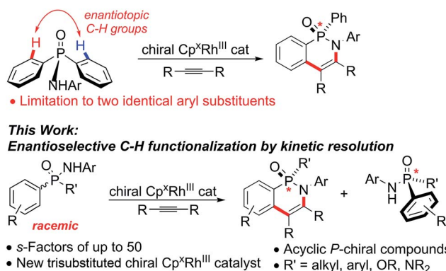
Scheme 1 Rh III -catalyzed desymmetrization and kinetic resolution approaches for the synthesis of P-chiral compounds.
