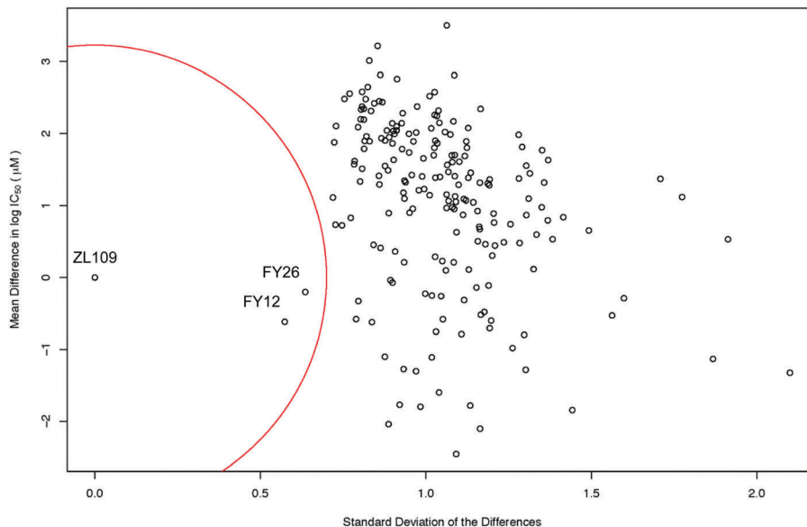
Fig. 3 Scatter plot of the mean difference in log IC_{50} values ( \mu\text{M} ) between all screened drugs and complex 2 (ZL109) vs. the SD of these differences. The red circle of radius 0.7 standard deviations denotes a 'region of significant similarity where the mean difference and standard deviation are low. The similarity with two osmium arene complexes which share the same chelated azopyridine ligand (complexes 3 (FY26) and 4 (FY12), Fig. 1) is evident.
