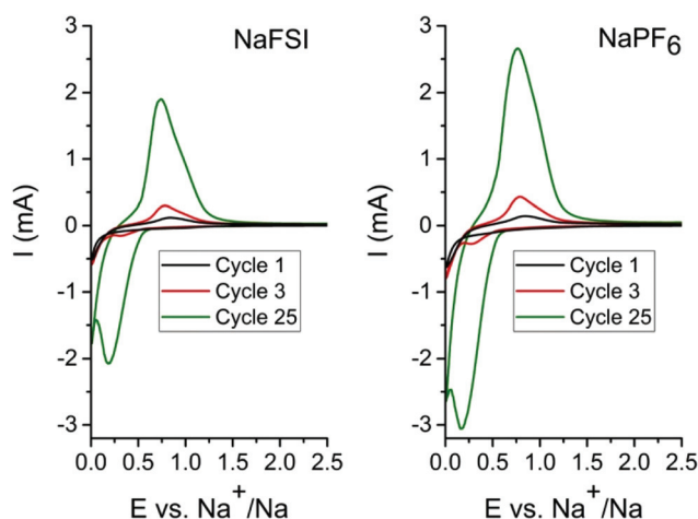
Fig. 1 Cyclic voltammogram of \text{Sn}_4\text{P}_3 vs. sodium metal using electrolytes of 1 M NaFSI (left) or \text{NaPF}_6 (right) dissolved in EC:DEC (1:1) and 10 vol% FEC additive. Scan was performed between 0.01 V–2.5 V at 1 \text{ mV s}^{-1} scan rate.
