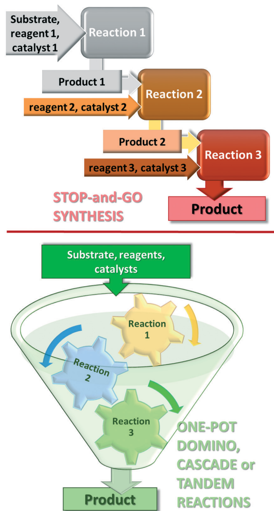
Fig. 1 Schemes of the stop-and-go and one-pot domino, cascade or tandem synthesis procedures.
