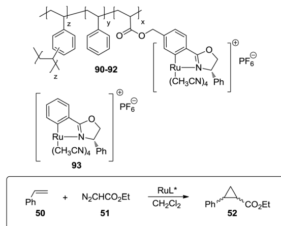
90 , x/y/z 1:100:10 (macroporous), TOF of 3.034\text{ h}^{-1} , cis:trans : 88:12, 94% ee 91 , x/y/z 1:55:55, (macroreticular), TOF of 1.265\text{ h}^{-1} , cis:trans : 82:18, 84% ee 92 , x/y/z 1:100:10, (i: ligand polymerization; ii: complexation), TOF of 1.102\text{ h}^{-1} , cis:trans : 83:17, 74% ee 93 , TOF of 2.694\text{ h}^{-1} cis:trans : 90:10, 98% ee
