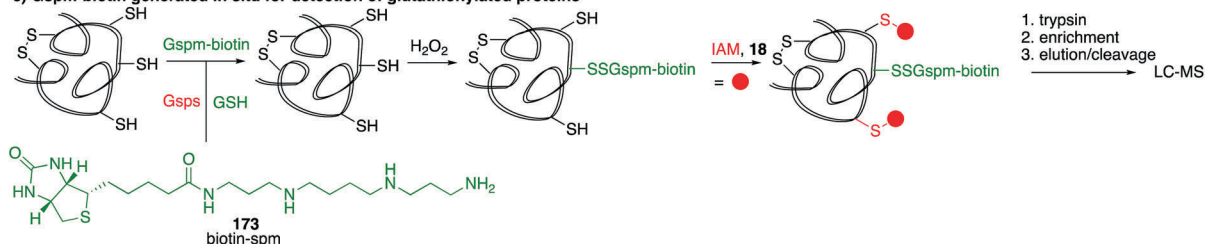
Fig. 22 (a and b) Biotin labelled GSH ( 171 ) or GSSG ( 172 ) can be fed to cells and incorporated into proteins. Affinity enrichment allows the proteins to be isolated and characterised further. (c) Biotin-spm ( 173 ) can be incubated with cells and using the enzyme GspS, can form an amide bond with GSH in situ . This biotin labelled GSH derivative can then react with glutathione reactive cysteines, followed by blocking of free thiols with 18 and subsequent detection.
