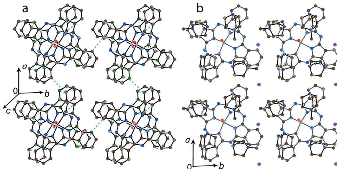
Fig. 8 (a) View of the phthalocyanine layer composed of the \pi -stacking [\{\text{Ti}^{\text{IV}}\text{O}(\text{Pc}^{3-})\}^-]_2 dimers in 13 . Short van der Waals C...C,N...C,N contacts are shown by green dashed lines. (b) Projection of the (\text{MDABCO})_2^- (\text{I}^-) layer on the phthalocyanine layer. Only one phthalocyanine from the dimer is shown (bonds are shown in grey). Salt 14 is isostructural to 13 .
